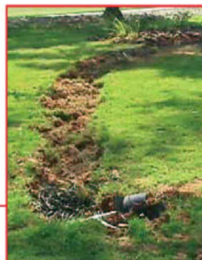
The lightning caused a surge to be induced into an underground coaxial cable, causing a trench to be formed. The surge traveled on the cable towards the subscriber's home.
