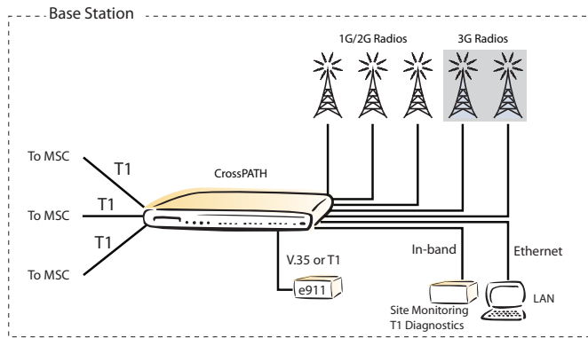
CrossPATH 4 and 3G support high-density base station growth and new services.
