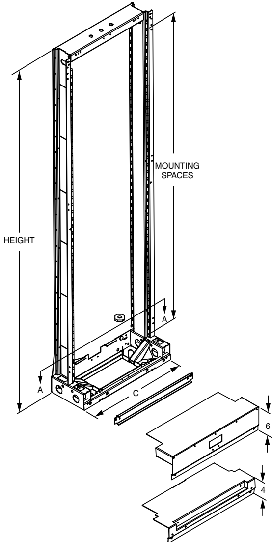
CLOSED BAY (GUARD BOX ON WIDE FLANGE)
