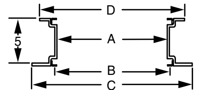
UPRIGHT PROFILE (NOTE 1)
